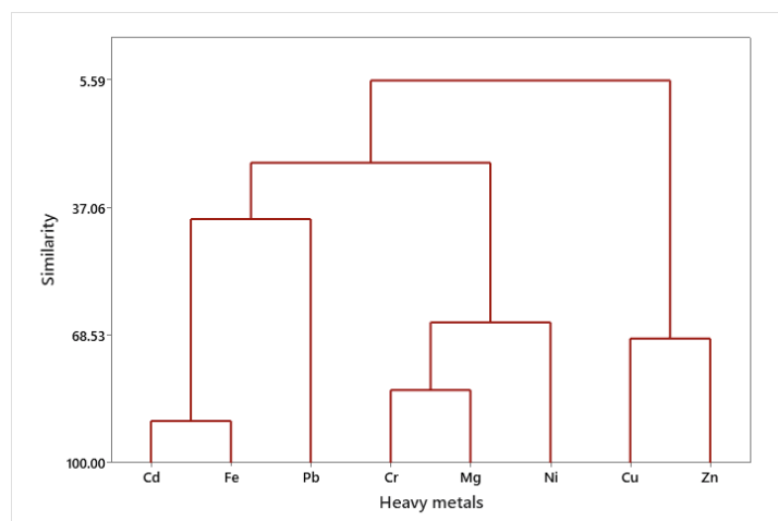
Fig. 7: Wet season Dendrogram for Heavy Metals in Tympantonus fuscatus
