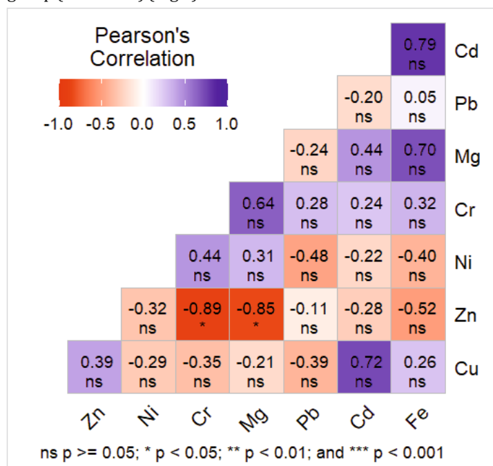
Fig. 6: Wet season Heavy metal correlation in the flesh of Tympantonus fuscatus
